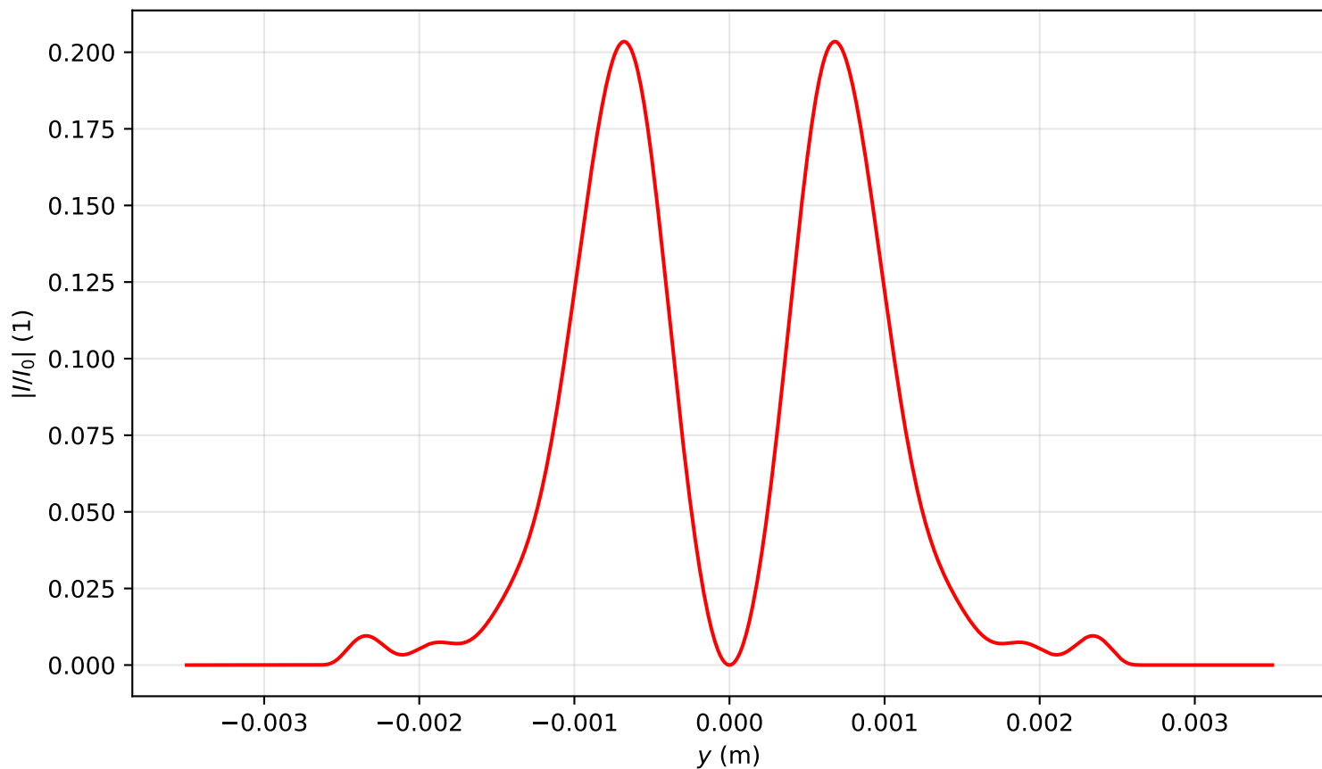
Intensity profile I(x=0, y, z=2.786)/I_0 , P_{in}=4.0P_{cr} , artificial time
